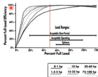
Electric motor
