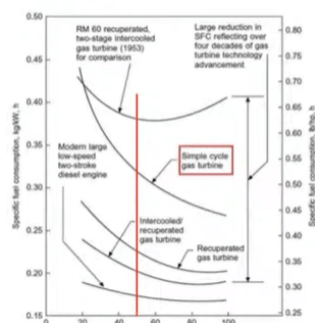
Prime mover
